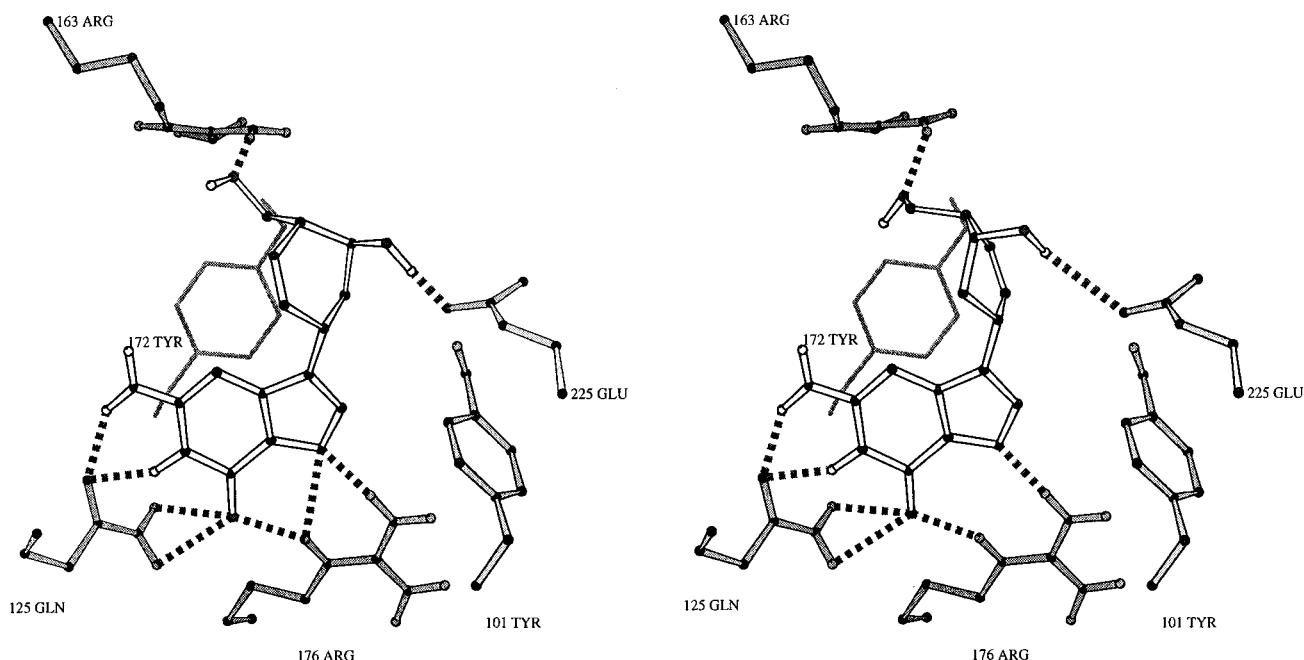
Figure 4. Plot of the minimized structure of HSV-1 thymidine kinase in complex with 4 (left) and 6 (right). Hydrogen bonds are plotted if the distance donor-hydrogen to acceptor is less than 2.7 Å and are marked by dotted lines. In the complex with 4 , the double bond in the sugar points to the front, while in the complex at the right, this double bond points to the back.
